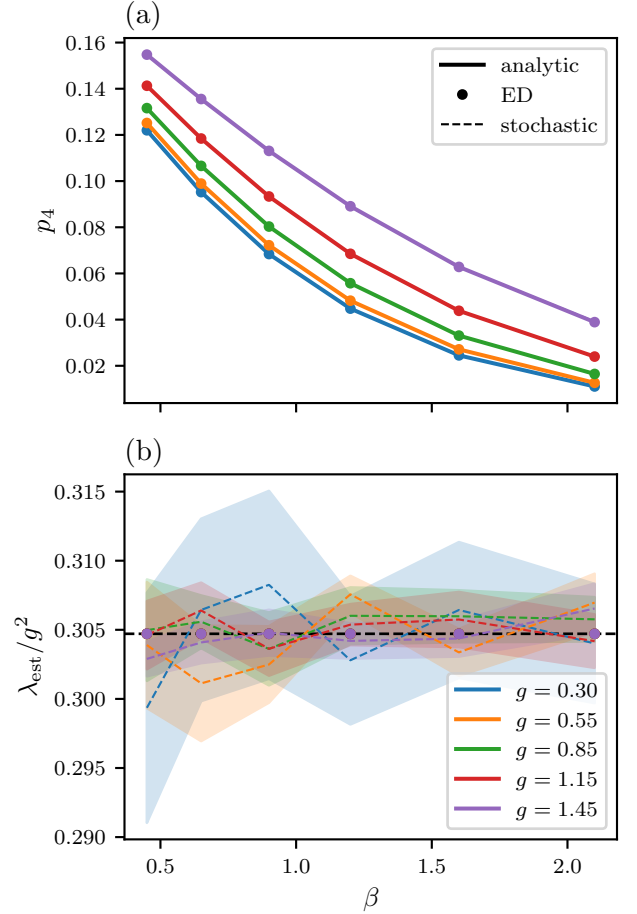
FIG. 2. Temperature dependence and scaling. (a) Population of the coupled state ( |4\rangle ) vs \beta for various couplings g . Circles (ED) match solid lines (analytic). (b) The extracted reorganisation energy \lambda_{\text{est}} collapsed by g^2 vs \beta . All curves hover near the theoretical thermodynamic limit (dashed lines), verifying that the bath's effect reduces to a single reorganisation energy \lambda .
