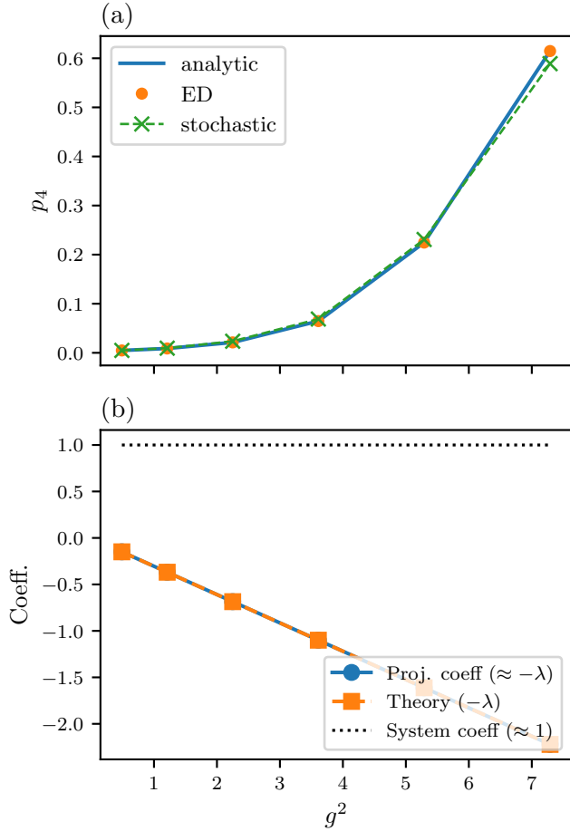
FIG. 3. Strong-coupling benchmark. (a) Population p_4 vs g^2 at fixed \beta , showing excellent agreement over the full range. (b) Coefficients of the HMF in the system basis vs g^2 . The projector component P = |4\rangle\langle 4| scales as -\lambda (orange/blue), while H_S remains unrenormalised (dotted), confirming H_{MF} = H_S - \lambda f^2 .
